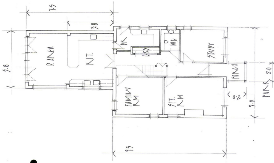
PROPOSED GROUND FLOOR PLAN 1:100
